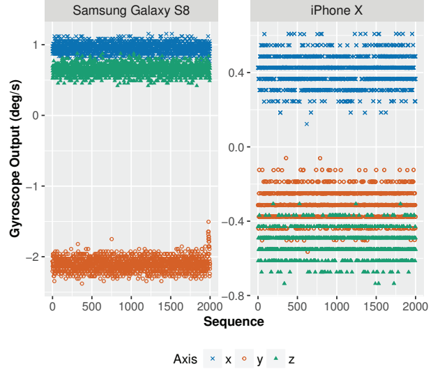
(a) Raw gyroscope measurements
