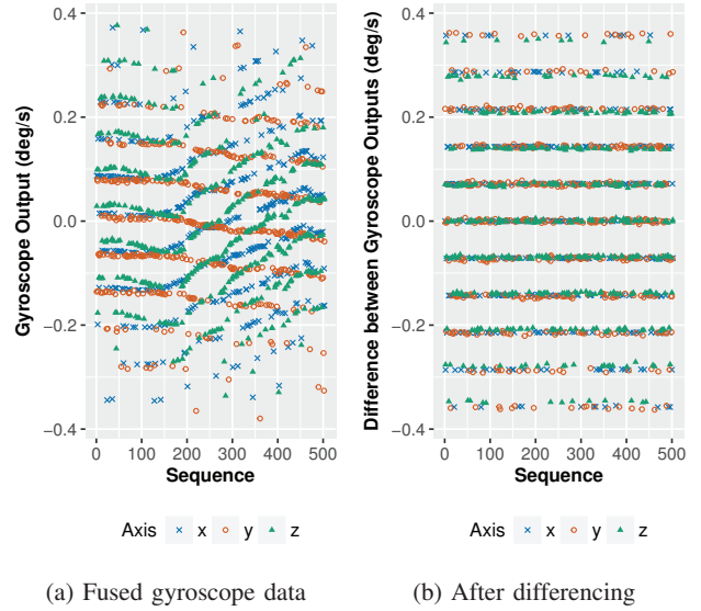
Fig. 4: Gyroscope data collected via JavaScript (iPad Air)
