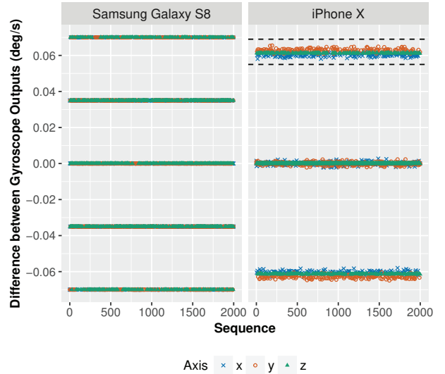
(b) Consecutive differences between gyroscope measurements
