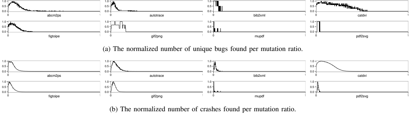
Fig. 5: The effectiveness of fuzzing per mutation ratio evaluated over 1,000 mutation ratios from 0.001 to 1.000.
